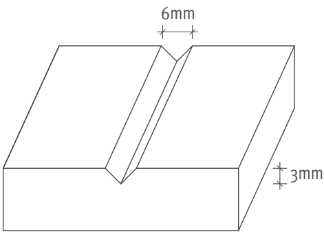
Standard Panel Groove Detail
